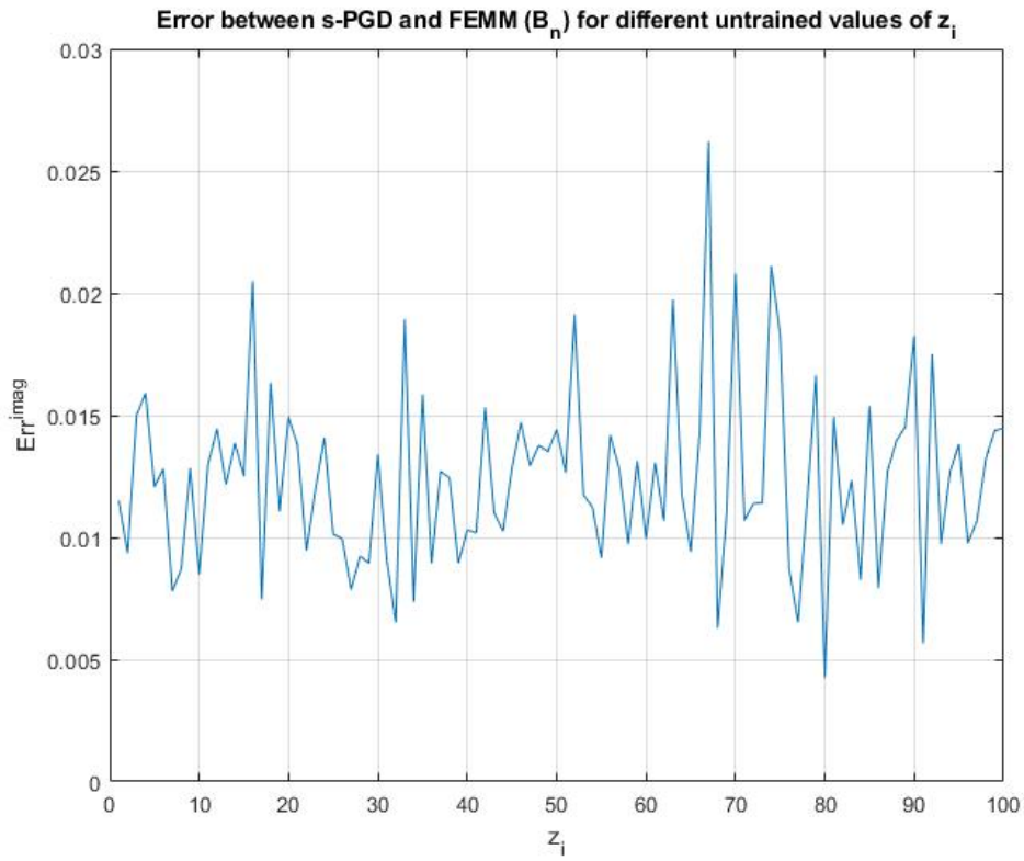
Figure 4.26 – Relative error of the s -PGD model (nonlinear B-H relationship) to determine the imaginary part of B_n for different untrained z_i . Error criteria of Eq. (4.26) is used.
