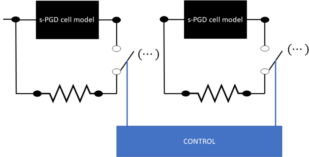
Figure 7.38 – Diagram of the cell balancing strategy employed in Section 7.6.5.
