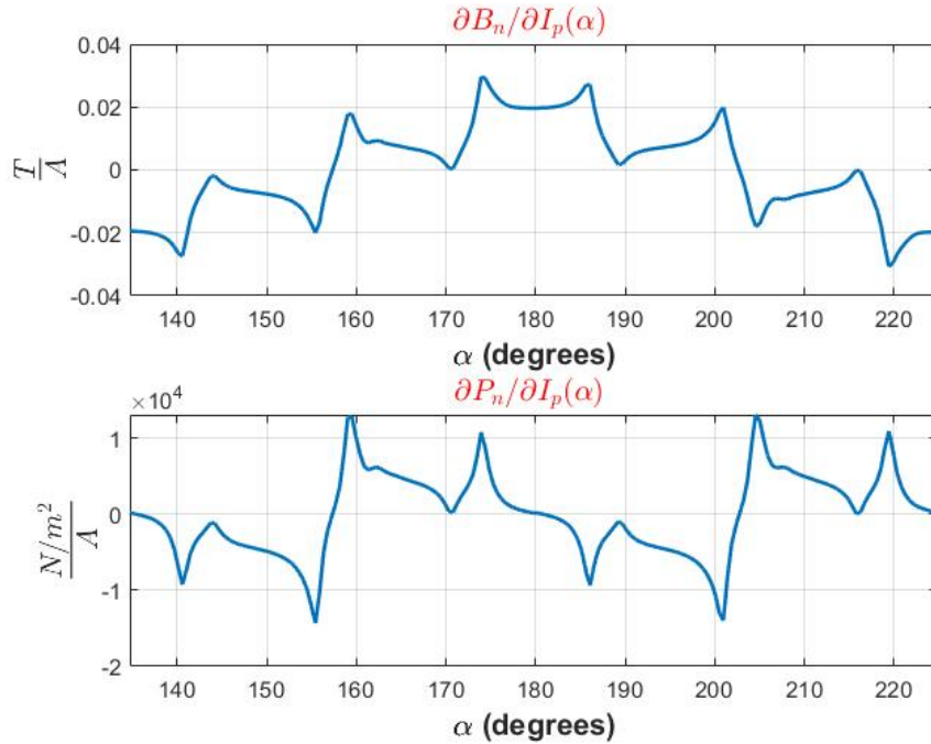
Figure 4.32 – Sensitivity of B_n and P_n for small changes in I_p . Operating point: \gamma = 0 degrees, I_p = 0.5 A, \tau = \pi/2 rad, \rho = 0 .
