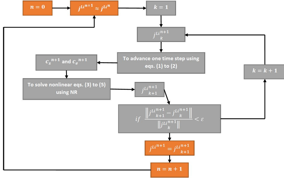
Figure 7.5 – Improved scheme to solve the electrochemical model.
