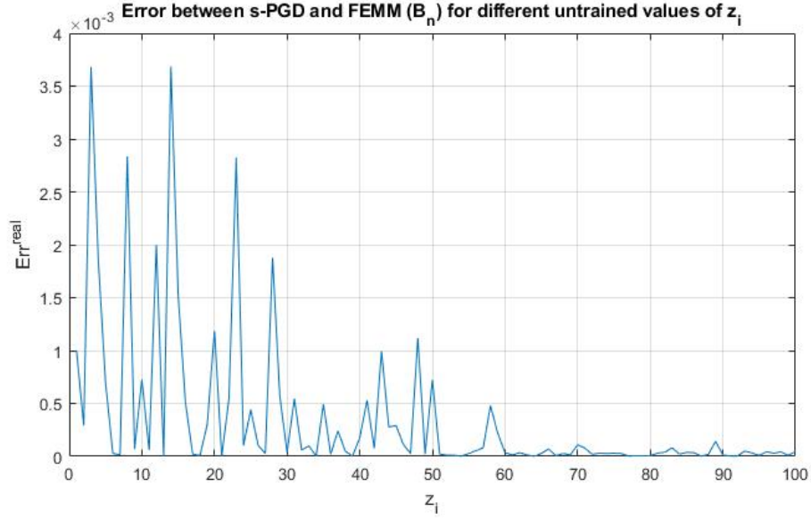
Figure 4.21 – Relative error of the s -PGD model (linear B-H relationship) to determine the real part of B_n for different untrained \mathbf{z}_i . Error criteria of Eq. (4.26) is used.
