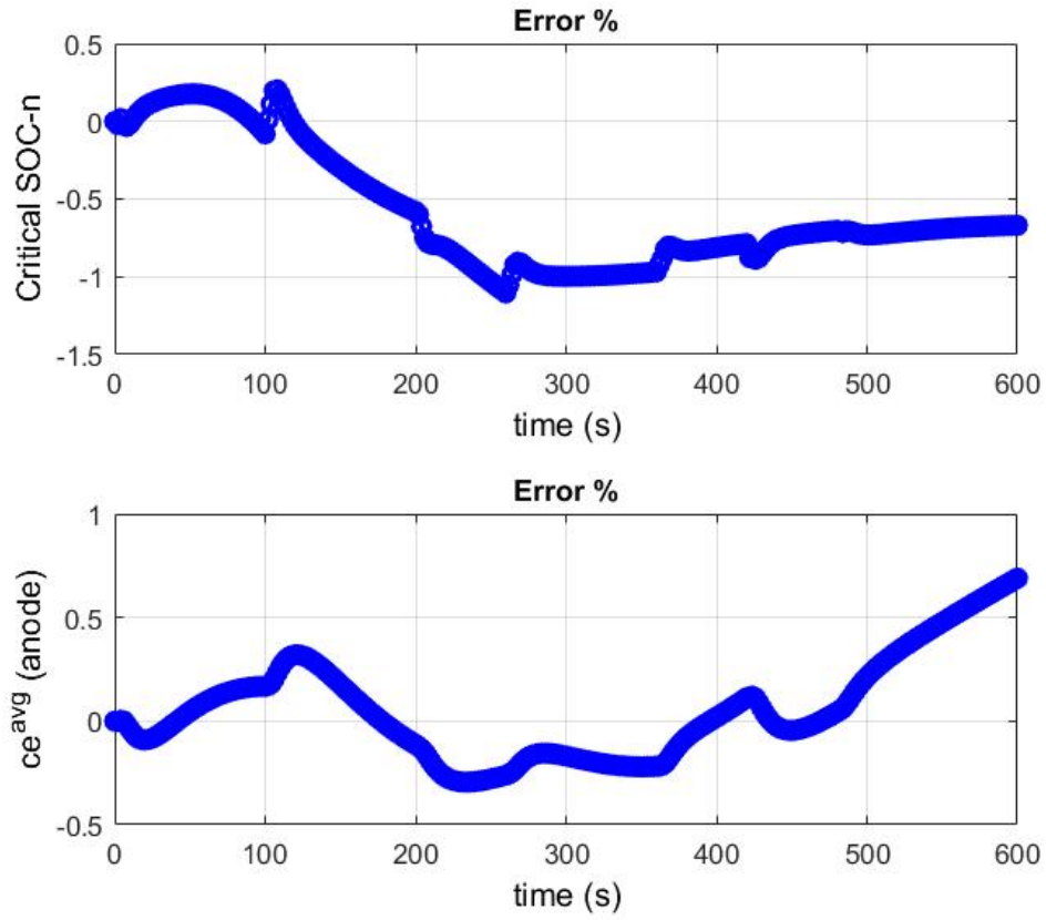
Figure 7.19 – Error between the s -PGD model and the POD model in a 10 minute itinerary (critical SoC and c_e^{\text{avg}} ). The s -PGD model is extracted based on itineraries of 10 minutes. \Delta t = 2s .
