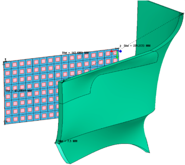
Figure 5.3 – Radar antenna and radome.
