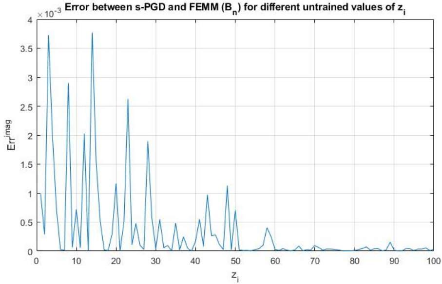
Figure 4.22 – Relative error of the s -PGD model (linear B-H relationship) to determine the imaginary part of B_n for different untrained \mathbf{z}_i . Error criteria of Eq. (4.26) is used.
