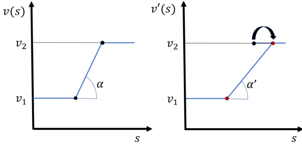
Figure 7.30 – Smoothing procedure of the reference driving cycle taken by the control v(s) when high discharge/charge rates happens when accelerating. This is used by the second step (See Algorithm 2) of the general procedure to adapt the driving cycle. v(s) and \alpha refers to the values before the modification and v'(s) and \alpha' refers to the values after the modification.
