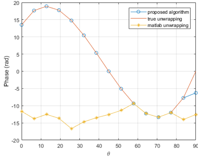
Figure 2.5 – Comparison of the proposed unwrapping procedure and the standard unwrapping function implemented in Matlab, in a coarse mesh consisting of 15 nodes.
