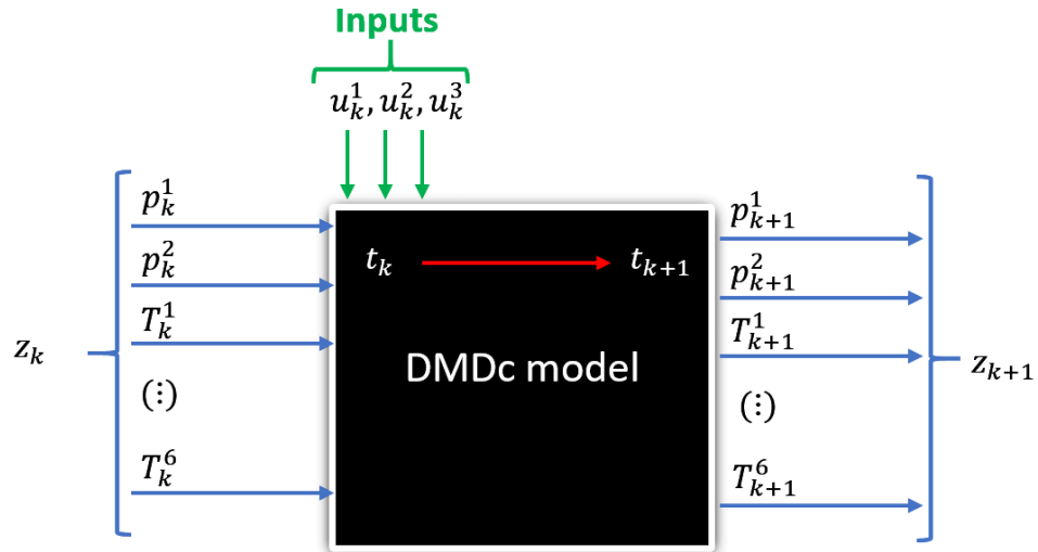
Figure 6.3 – Diagram illustrating the inputs and the state vector of the proposed DMDc model to reproduce the pruned data of the system.
