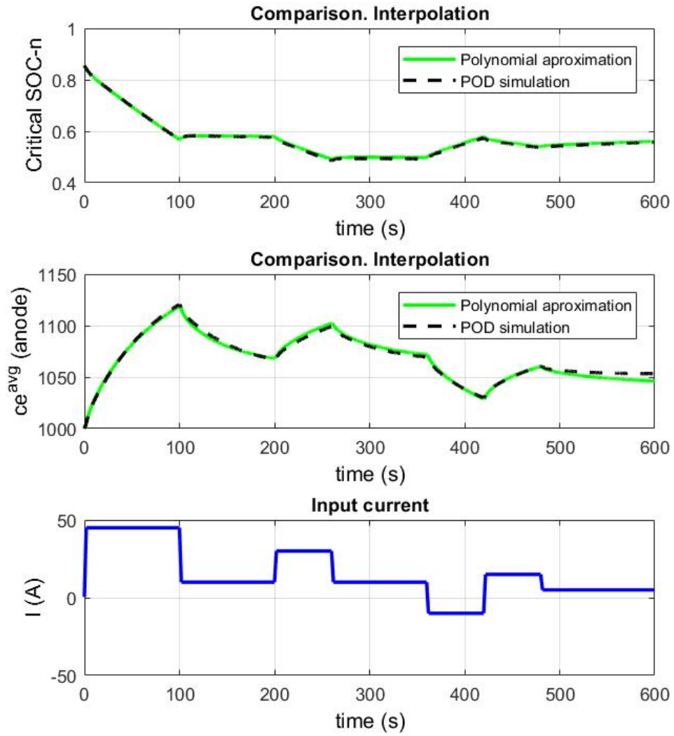
Figure 7.18 – Comparison of the results between the s -PGD model and the POD model in a 10-minute itinerary (critical SoC and c_e^{\text{avg}} ). The s -PGD model is extracted based on itineraries of 10 minutes. \Delta t = 2s .
