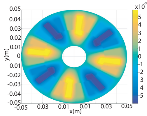
(b) i_a = 0 A, i_b = 0 A, i_c = 0 A, B_r = 1.01 T and \rho = 10^\circ
