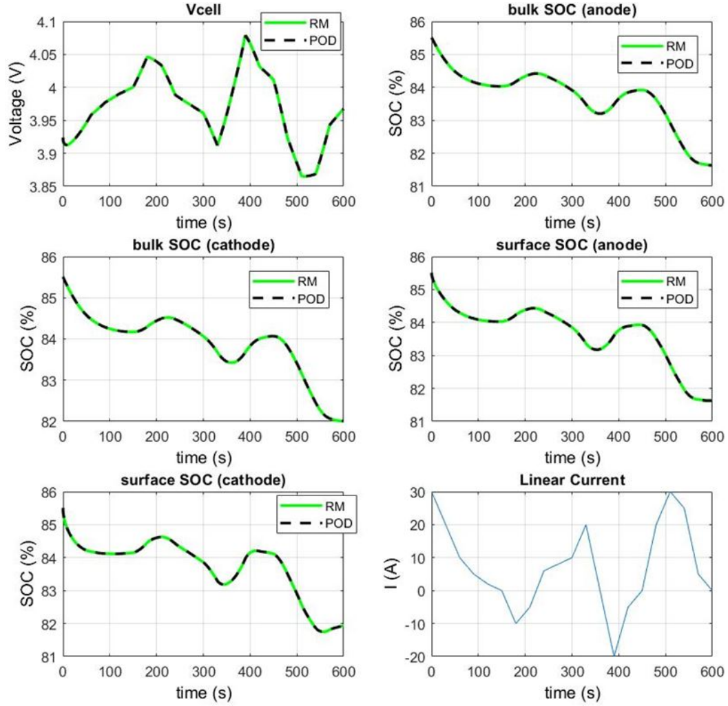
Figure 7.8 – Comparison of full- and reduced-order simulations of the second cell. . The different SoC and the cell voltage are compared and the input current used during the simulation is shown in the last picture. Legend: RM = Results of the full P2D model; POD = Results of the POD model.
